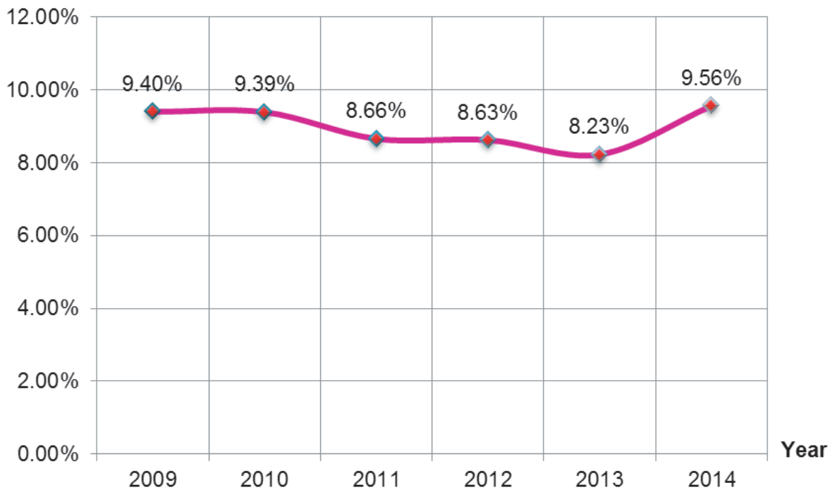
Figure 8: System Losses in Phnom Penh System from 2009 to 2014
